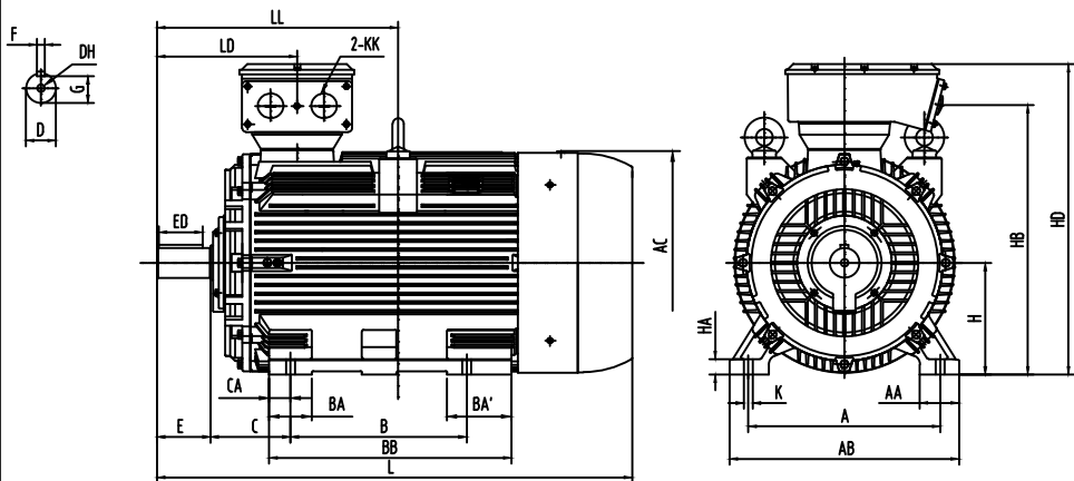
OUTLINE DIMENSIONS FOOT MOUNTED MOTORS
