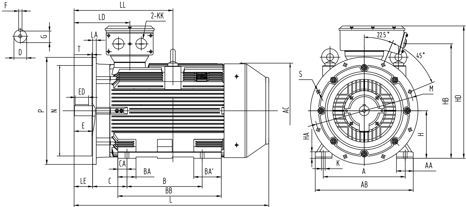
OUTLINE DIMENSIONS FOOT MOUNTED MOTORS
