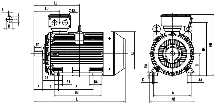
OUTLINE DIMENSIONS FOOT MOUNTED MOTORS
