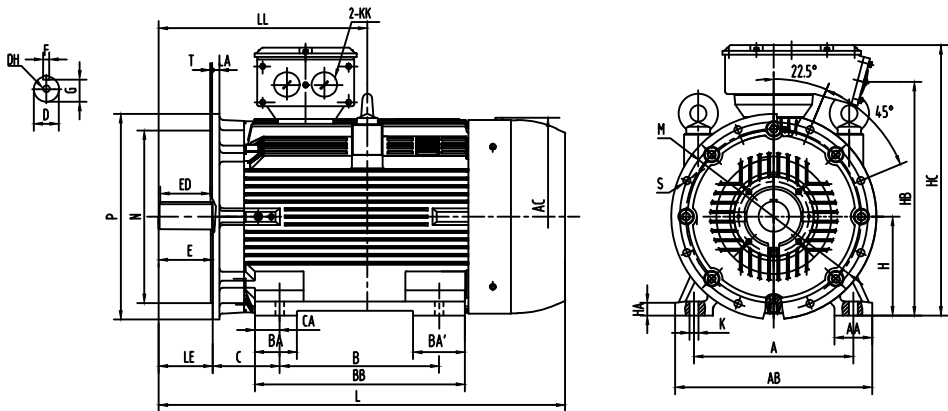
OUTLINE DIMENSIONS FOOT-FLANGE MOUNTED MOTORS
