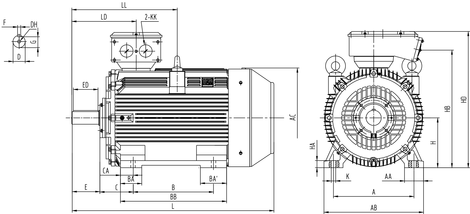
OUTLINE DIMENSIONS FOOT MOUNTED MOTORS
