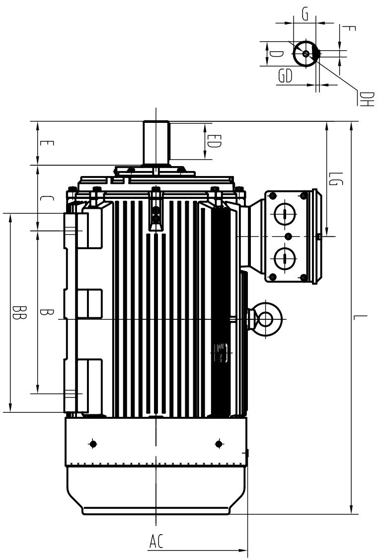
OUTLINE DIMENSIONS FOOT MOUNTED MOTORS
